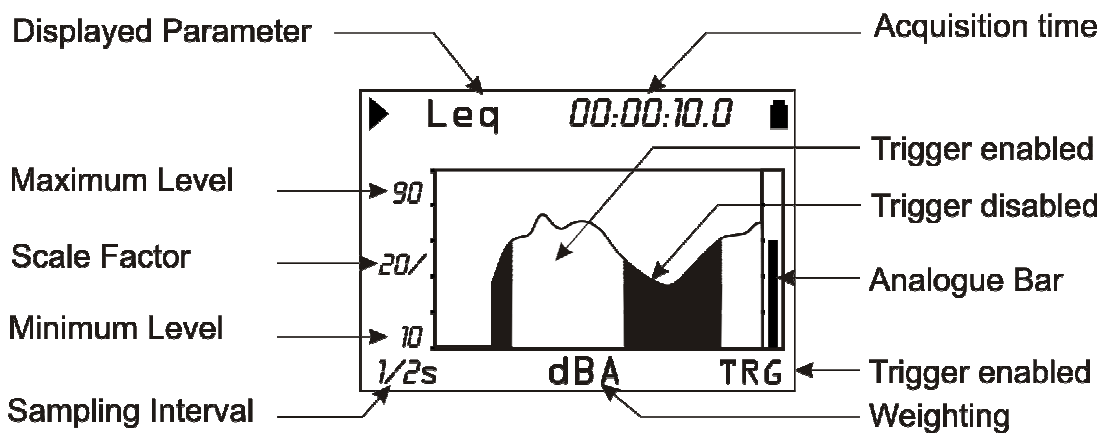
Fig. 26 - Description of the "Event trigger" display"
