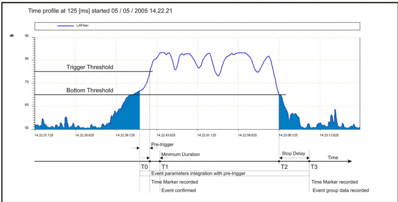
Fig. 25 - Description of the event trigger parameters
