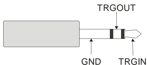
Fig. 1 - TRIGGER stereo connector.
