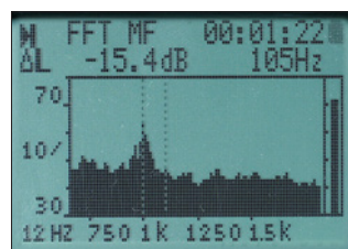
FFT narrow band spectrum (option FFT)
