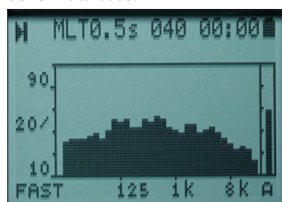
Third octave bands spectrum (option HD2110.O1)
