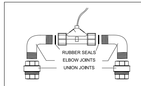
TYPICAL IN-LINE ASSEMBLY FOR HI7635 (or HI7636).
